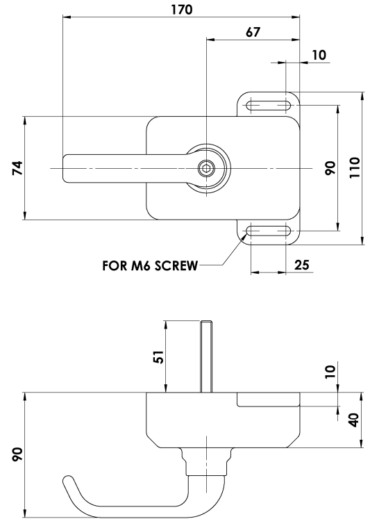
Product Dimensions – Type: UGB Rotary Rear Handle
